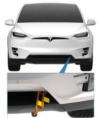
Opening hood from outside without 12-volts:
